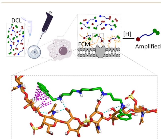
Fig. 11 Schematic representation of live-cell-templated DCC experiment targeting the GAGs of the ECM. The inset shows a model interaction between the amplified member of the library ( 11a ) and chondroitin sulfate A (CDS-A), the main GAG in the ECM of A549 cells used for the DCC experiments. In the model, non-polar H atoms are omitted, CDS-A and 11a are represented with orange and green C-atoms, respectively. On the other hand, H-bonds and CH- \pi interactions are depicted with blue and pink dashed lines, respectively.
