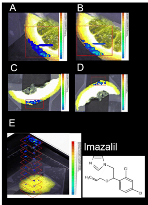
Fig. 10 Positive-ion LAESI-TOF-MSI accurate ion maps of (A, C) the ^{35}\text{Cl}^{35}\text{Cl} isotope [\text{M} + \text{H}]^+ ion at m/z 297.056 ( \pm 5 mDa), and (B, D) the ^{35}\text{Cl}^{37}\text{Cl} isotope [\text{M} + \text{H}]^+ ion at m/z 299.056 ( \pm 5 mDa), on (A, B) orange slice and (C, D) lemon slice, showing the spatial distributions of the post-harvest fungicide imazalil. (E) 3D profiling of imazalil in a lemon-peel slice, represented by a stack of 2D ion maps of m/z 297.055. Figure adapted and reprinted from ref. 17 with permission from Springer Nature, copyright (2014).
