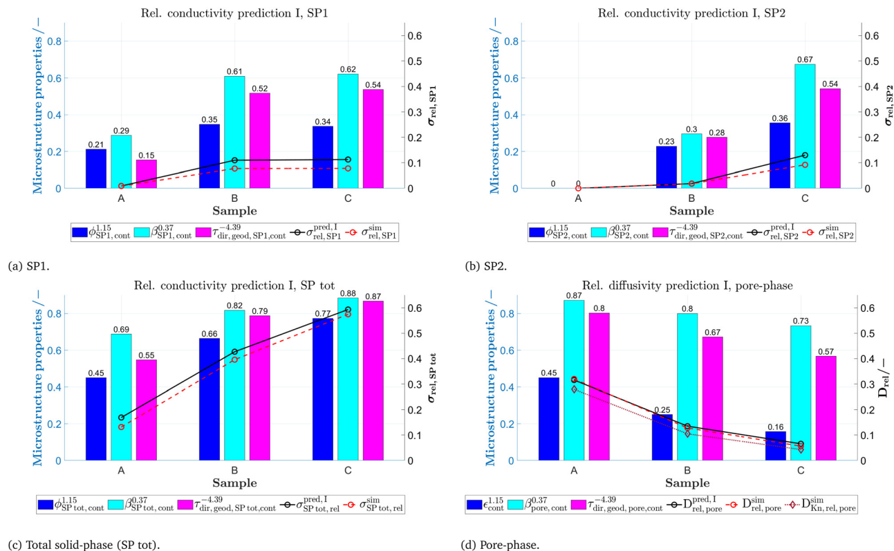
Fig. 24 M -factor prediction I (black lines) and its three components (volume fraction effect \phi^{1.15} , constricitivity effect \beta^{0.37} and tortuosity effect \tau_{dir, geod}^{-4.39} ) and simulated M -factors (red lines), for (a) SP1, (b) SP2, (c) total solid-phase (SP tot) and (d) the pore-phase of the sphere-packing structures. The used variables are summarized in the Tables 9 and 10.
