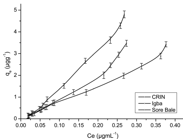
Fig. 11 Desorption isotherms of \alpha -endosulfan for CRIN, Igba and Sore Bale farm soils, where q_e = concentration of \alpha -endosulfan undesorbed at equilibrium ( \mu\text{g g}^{-1} ), C_e = concentration of \alpha -endosulfan desorbed into 0.01 M \text{CaCl}_2 at equilibrium ( \mu\text{g mL}^{-1} ).
