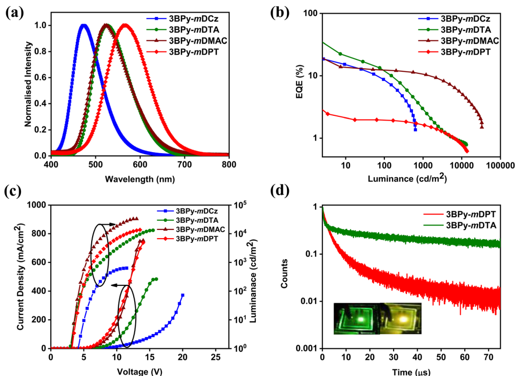
Fig. 5 (a) EL spectra; (b) EQE versus luminance characteristics (c) luminance–voltage–current density characteristics. (d) Transient EL spectra; inset is an EL illumination image of 3BPY-mDTA (green emission) and 3BPY-mDPT (yellow emission).
