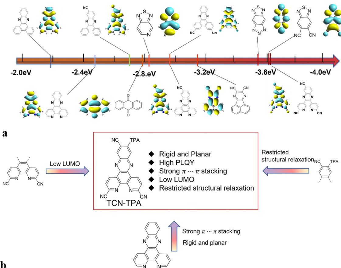
Scheme 1 (a) Comparison of the LUMO levels of various acceptors applied for TADFs and calculated with B3LYP/6-31G(d); (b) the chemical structure and molecular design strategy of TCN-TPA.
