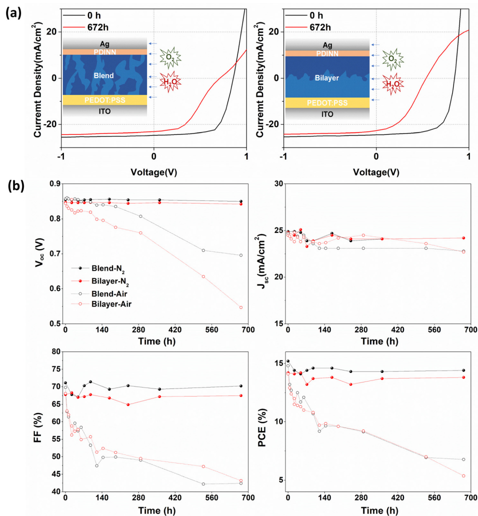
Fig. 4 (a) Scheme of water and O 2 diffusion into the OSC, and the corresponding J-V curves with blended and bilayer PALs stored in air. (b) Performance evolution of OSCs with blended (black curve) and bilayer (red curve) PALs stored in a glovebox (N 2 – solid curve) and fume hood (air – dashed curve) for 672 hours.
