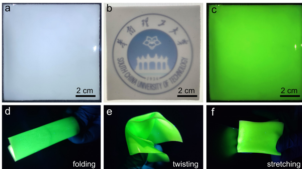
Fig. 4 (a) and (b) Photographs of large-sized and transparent Cs 2 ZnBr 4 :25%Mn 2+ @PDSM thin film under visible light. (c) Photograph of Cs 2 ZnBr 4 :25%Mn 2+ @PDSM thin film under 365nm UV light. Photographs of the flexible Cs 2 ZnBr 4 :25%Mn 2+ @PDSM thin film at different mechanical deformations under UV excitation: folding (d), twisting (e), and stretching (f).
