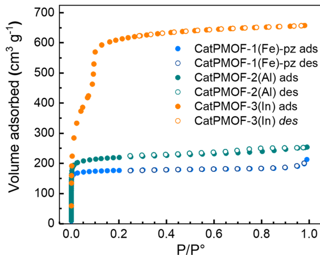
Fig. 10 Nitrogen sorption isotherms recorded at 77 K, evidencing that all phases are porous.
