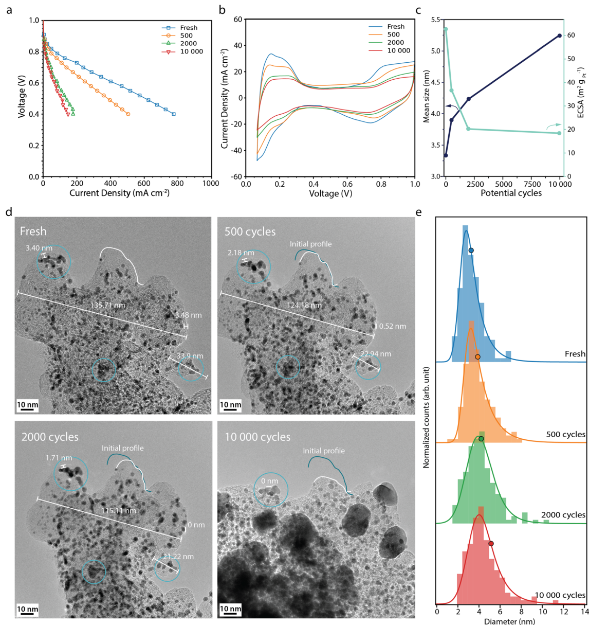
Fig. 3 (a) Polarisation curves measured potentiostatically, and (b) cyclic voltammograms recorded at 100 mV s -1 recorded for the fresh fuel cell and after 500, 2000 and 10 000 start-up shutdown AST potential cycles. (c) Mean Pt particle size (black) and the electrochemically active surface area, ECSA (light blue) versus the number of potential cycles. (d) Corresponding IL-TEM images and (e) corresponding Pt particle size distributions. The histograms, from 150 Pt particles at each point in time, are fitted with an exponentially modified Gaussian function, and the mean diameter is marked with a circle. The x-axis of histograms shown here is limited to <14 nm, but it is important to note that larger particles (>20 nm) are observed after extensive ageing. The full set of Pt particles is used to calculate the mean size and the full histograms can be found in Fig. S4.†
