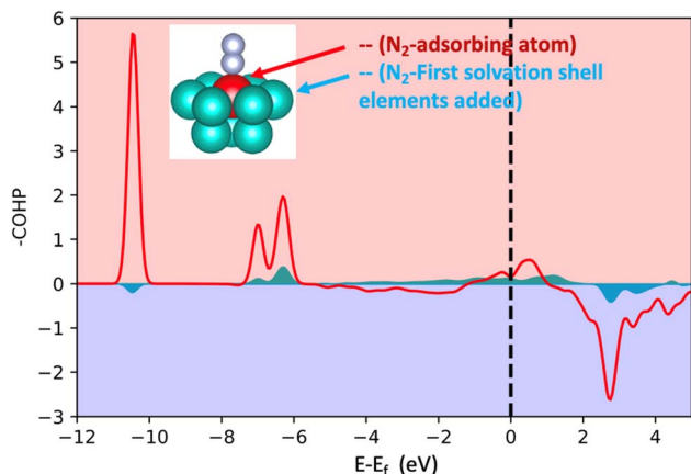
Fig. 4 Projected crystal orbital Hamiltonian population ( -pCOHP ) analysis for the bonds between N 2 and the adsorbing atoms and between N 2 and the first solvation shell. The used model is shown in Fig. 2 (the case of 16 atoms). The red represents the summed-up interactions between N 2 and the adsorbing element while light blue represents summed pairs of elements from the first solvation shell and N 2 .
