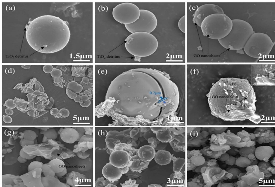
Fig. 14 (a0) Schematic illustration of the method for creating GO/TiO 2 /paraffin microcapsules, SEM images of (a and b) TiO 2 /paraffin microcapsules, (c and d) GO/TiO 2 /paraffin microcapsules containing 1 wt% GO, (e–g) GO/TiO 2 /paraffin microcapsules containing 2 wt% GO, and (h and i) GO/TiO 2 /paraffin microcapsules containing 3 wt% GO. 163 Reproduced with permission from ref. 163 Copyright 2021 Elsevier.
