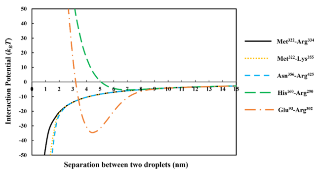
Fig. 3 The interaction potentials, plotted against the inter-droplet separation distance, resulting from the overlap of adsorbed layers of five different soy-derived polypeptides ( i.e. Met 322 –Arg 334 , Met 322 –Lys 355 , Asn 356 –Arg 425 , His 160 –Arg 290 and Glu 93 –Arg 302 ) respectively. The diameter of oil droplets was taken as 1 \mu\text{m} . The results are produced at a background electrolyte volume fraction of 0.01 (roughly equals to 100 mM NaCl) and at pH = 5.5. The more direct van der Waals attraction between the droplets have also been included in these calculations.
