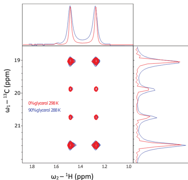
Fig. 5 In order to simulate the rotational environment of the labelled amino acid inside a protein, L- [\alpha\text{-}^2\text{H}, ^{15}\text{N}, \beta\text{-}^{13}\text{C}] -alanine was dissolved in a viscous glycerol medium and studied by NMR. The figure shows the ^{13}\text{C} - ^1\text{H} decoupled HSQC experiment of the sample in ^2\text{H}_2\text{O} at 298 K (red) and 90 vol% glycerol at 288 K (blue trace). Under 0 vol% glycerol, the ratio of intensities is 3 : 1 : 1 : 3, as expected for a small molecule. At 90 vol% glycerol and low temperature, the resonances remained intense. The intensity ratio changed to approximately 2 : 1 : 1 : 2. Due to the outer resonances having 9\times faster relaxation than the inner lines, in the macromolecular limit when the molecule tumbles slowly. Although the effects of slow tumbling are clear, the resonances remain sharp indicating the utility of this reagent inside high molecular weight proteins.
