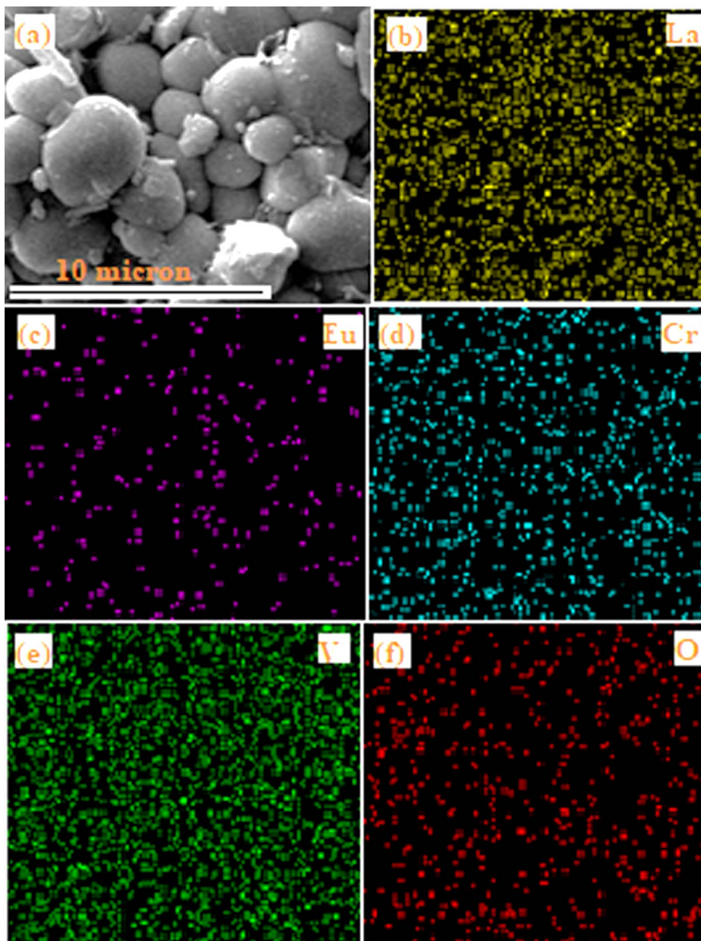
Fig. 5 Elemental mapping and distribution of the component elements present in the \text{LaVO}_4\text{:1Eu}^{3+}\text{:0.1Cr}^{3+} phosphor: (a) selected area used for elemental mappings, (b) La, (c) Eu, (d) Cr, (e) V and (f) O elements.
