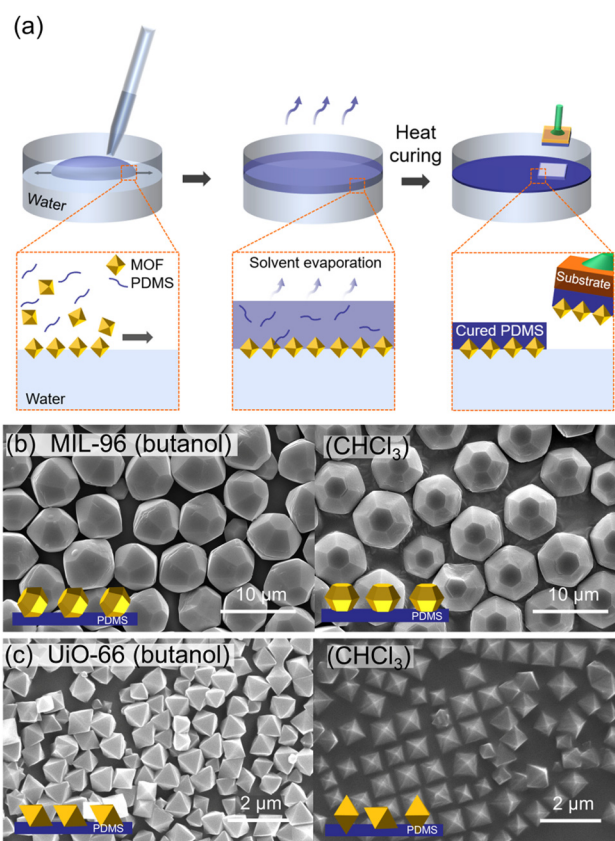
Fig. 16 (a) Scheme of preparation of oriented MOF–PDMS films. (b) SEM images of oriented (b) MIL-96–PDMS films and (c) UiO-66–PDMS films prepared using butanol (left) and CHCl_3 (right) as a casting solvent. Adapted with permission from ref. 101. Copyright 2021, American Chemical Society.
