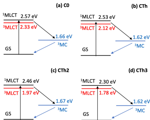
Fig. 8 Computed Jablonski diagrams of the important excited states in (a) C0 , (b) CTh , (c) CTh2 and (d) CTh3 . Using TDDFT, the energies of the ^1\text{MLCT} states were computed at the ^3\text{MLCT} optimized geometry and the energies of the ^3\text{MC} was computed at the ^3\text{MC} optimized geometry ( ^1\text{MLCT} and ^3\text{MLCT} states have similar geometries). Both geometries were computed using UKS and the relevant geometries are in the ESI.†
