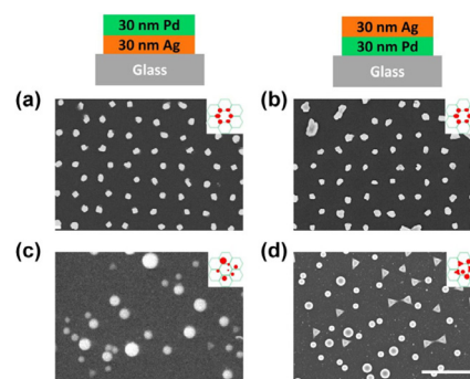
Fig. 6 SEM images of Pd/Ag/Glass honeycomb array after (a) thermal annealing and (c) applying five 100 mJ cm −2 pulses. Ag/Pd/Glass honeycomb array after (b) thermal annealing and (d) applying five 100 mJ cm −2 pulses. The scale bar is 1 \mu m and applies to all images.
