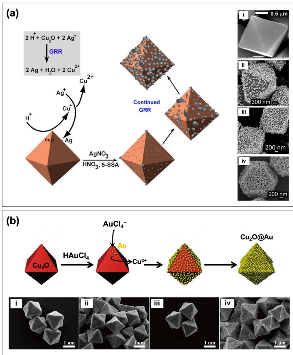
Fig. 4 Schematic depiction of the formation of (a) Cu 2 O@Ag and (b) Cu 2 O@Au core-shell nanocomposites through GRR. Also shown are the SEM images of the structures produced with (i) no metal and (ii) to (iv) increasing loading amount of metal. Reproduced with permission from (a) ref. 69, copyright 2017 the Royal Society of Chemistry, and (b) ref. 62, copyright 2016 Elsevier.
