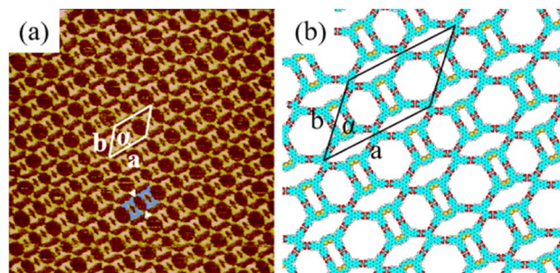
Fig. 3 (a) High-resolution STM image of the H 4 BDETP/H 4 BTB co-assembly structure at the 1-heptanoic acid/HOPG interface, I_{set} = 265.5 pA and V_{bias} = 754.4 mV ( 46.3 nm \times 46.3 nm). (b) The calculated molecular model for the H 4 BDETP/H 4 BTB co-assembly structure.
