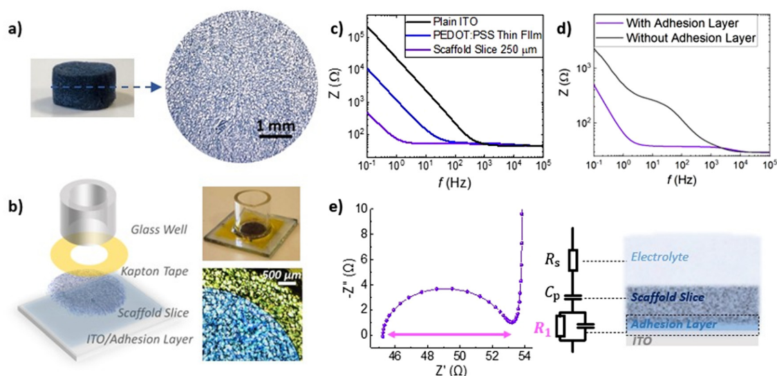
Fig. 3 (a) Digital pictures of a PEDOT:PSS scaffold and a 250 \mu\text{m} thick scaffold slice made of PEDOT:PSS crosslinked with PEGDE 3 wt%. (b) Schematic of the 3D bioelectronic device developed in this study and as shown in the digital picture on the top right. A top view of the edge of this device is shown in the bottom left microscope image. The electrochemical area of the device is well defined by the micro-patterned Kapton tape. (c) Impedance magnitude versus frequency plots for the devices bearing the same electrochemical area as defined by the Kapton tape with plain ITO (black), ITO/adhesion layer (blue) and with the scaffold slice attached (purple). (d) A typical impedance versus frequency plot obtained for a 3D device that uses and adhesion layer to electrically connect the scaffold slice on ITO (purple) and for 3D device without an adhesion layer used (grey). (e) A typical Nyquist plot of an optimized ITO/adhesion layer/scaffold slice device and the equivalent circuit model used to raw EIS data.
