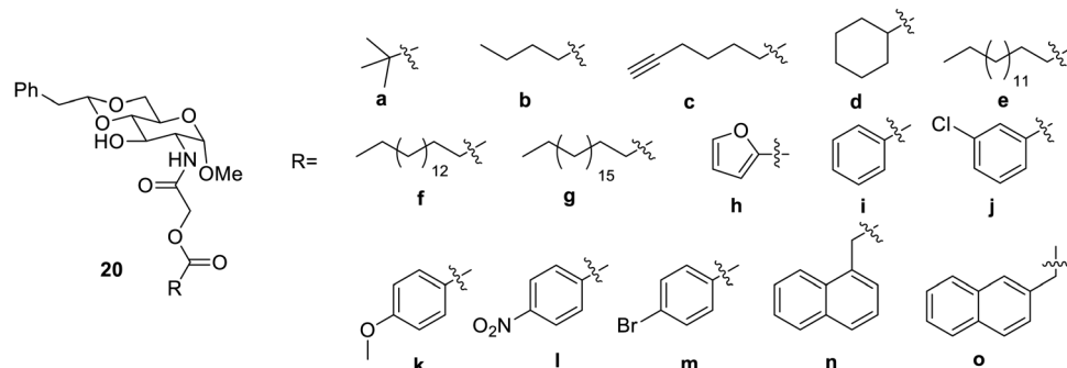
Fig. 12 Ester derivatives of the N -acetyl- \alpha -D-glucosamine.
