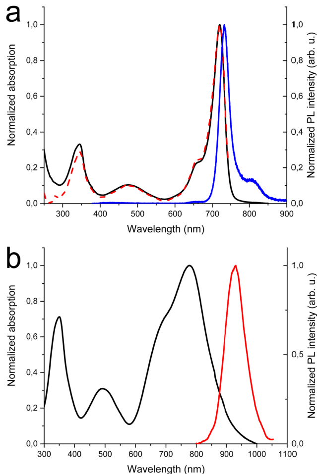
Fig. 1 (a) Absorption (black solid), excitation (red dash) and PL (blue solid) spectra of DTD PAB in chloroform ( c = 10^{-5} M), (b) absorption (black solid) and PL (red solid) spectra of DTD PAB cast film.
