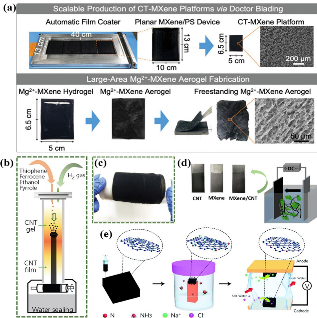
Fig. 9 (a) Illustration of the scalable fabrication of large-area Mg^{2+} -MXene aerogels, 159 reproduced with permission from Wiley. (b) Schematic diagram of the preparation of CNT film and (c) a digital photograph of the as-fabricated CNT film, reproduced from ref. 165 with permission from ICE publishing. (d) Digital photographs of the as-prepared freestanding electrodes and scheme of the electrophoretic deposition process, reproduced from ref. 161 with permission from Elsevier. (e) Schematic illustration of the fabrication of the N-doped GO/CNTs electrode and CDI cell, reproduced from ref. 167 with permission from the Royal Society of Chemistry.
