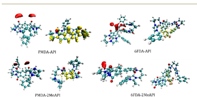
Fig. 11 The SDFs of anions (red) and cationic polymer chains (gold) around the positively charged polymer chain. The corresponding isovales for the anion and cationic species of number densities are 10 \text{ nm}^{-3} and 4 \text{ nm}^{-3} , respectively. The central positively charged polymer chain are represented as CPK models.
