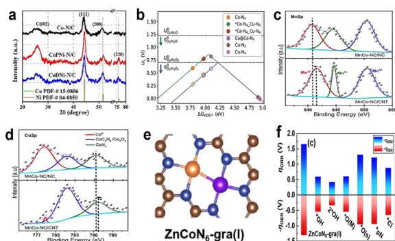
Fig. 17 (a) XRD patterns of Co–N/C, Co x Ni–N/C ( x = \text{P} and \text{D} ). 121 (b) The volcano plots for the four-electron ORR to H 2 O (solid circles) and two-electron ORR to H 2 O 2 (empty circles). 122 High-resolution (c) Mn 2p and (d) Co 2p spectra of MnCo–NC/NC and MnCo–NC/CNT. 123 (e) The most stable configuration of ZnCoN x –gra. 124 (f) The overpotential of the ORR and OER for ZnCoN 6 –gra (1) with or without electron-withdrawing functional groups. 124
