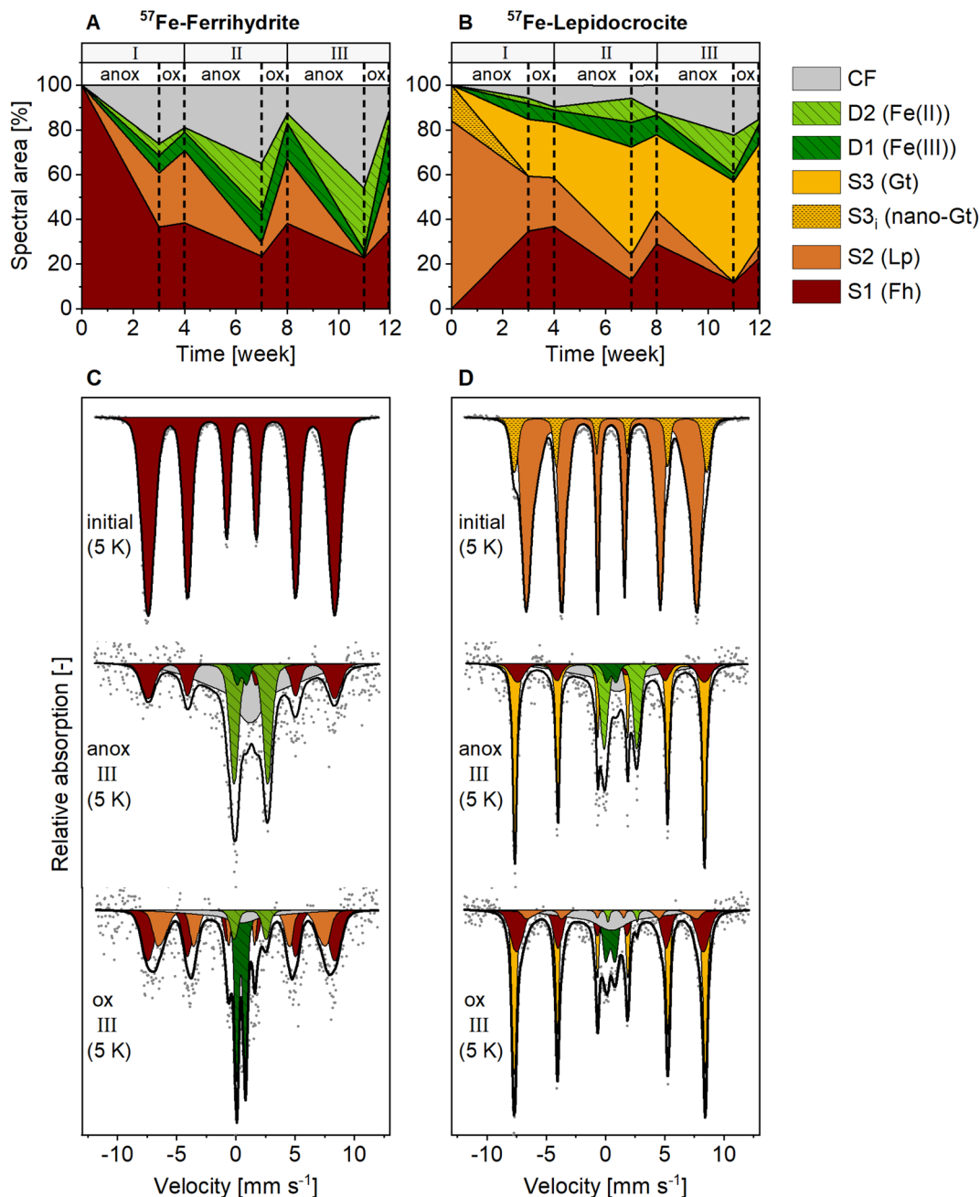
Fig. 4 Spectral area of fit components in 5 K Mössbauer spectra for (A) ^{57}\text{Fe} -ferrhydrite-soil mixes, and (B) ^{57}\text{Fe} -lepidocrocite-soil mixes incubated in the redox fluctuating mesocosms. Lower panels show Mössbauer spectra collected at 5 K from initial mineral-soil mixes containing (C) ^{57}\text{Fe} -ferrhydrite or (D) ^{57}\text{Fe} -lepidocrocite and corresponding samples after incubation in the redox fluctuating mesocosms, sampled in the anoxic (11 weeks) and oxic (12 weeks) period of redox cycle III. Abbreviations: anox = anoxic, ox = oxic, D = doublet, S = sextet, CF = collapsed feature, Fh = ferrhydrite, Lp = lepidocrocite, Gt = goethite. Goethite in initial ^{57}\text{Fe} -lepidocrocite likely was nano-crystalline. Interpretations of Mössbauer fit components are given in Table 1, fitting parameters are presented in Tables S9 and S10.†
