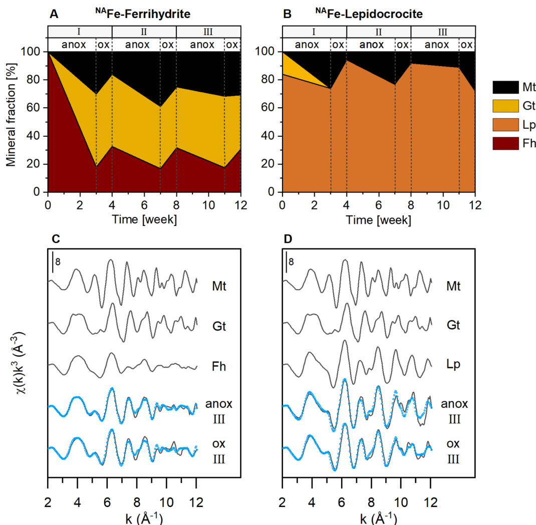
Fig. 2 Iron mineral fractions as determined by linear combination fitting of Fe K-edge EXAFS spectra in ^{NA}\text{Fe} -mineral samples from mesh bags without soil for (A) ^{NA}\text{Fe} -ferrihydrite and (B) ^{NA}\text{Fe} -lepidocrocite incubated for 12 weeks in the redox fluctuating mesocosms, with (C and D) reference spectra and spectra from redox cycle III. According to EXAFS data, the initial ^{NA}\text{Fe} -lepidocrocite contained minor fractions (16%) of goethite which was likely nano-crystalline (ESI Section S2†). All spectra and fits are presented in Fig. S15.† Fractions of fit components and reduced \chi^2 are presented in Table S4.† Abbreviations: Mt = magnetite, Gt = goethite, Fh = ferrihydrite, Lp = lepidocrocite, anox = anoxic, ox = oxic.
