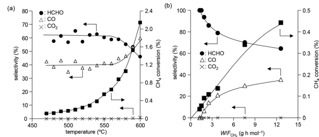
Fig. 4 (a) Product selectivity and \text{CH}_4 conversion as a function of reaction temperature with \text{O}_2 over \text{BiPO}_4 -DEG. Reaction conditions: \text{BiPO}_4 -DEG (100 mg), \text{CH}_4/\text{O}_2/\text{N}_2 (2/2/6 sccm). (b) Effect of W/F_{\text{CH}_4} on product selectivity and \text{CH}_4 conversion. Reaction conditions: \text{BiPO}_4 -DEG (100 mg), \text{CH}_4/\text{O}_2/\text{N}_2 (38 : 8 : 54 molar ratio; total 7.8–78 sccm), reaction temperature (550 °C).
