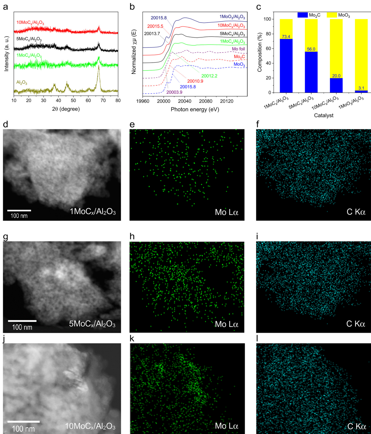
Fig. 3 (a) XRD patterns of Al_2O_3 and tested catalysts, (b) XAS spectra, and (c) linear combination fitting (LCF) results of supported MoC_x catalysts. MoO_3 , Mo_2C , Mo foil, and 1MoO_3/Al_2O_3 were included as the standards. Representative dark-field TEM images of (d) 1MoC_x/Al_2O_3 , (g) 5MoC_x/Al_2O_3 , and (j) 10MoC_x/Al_2O_3 and their EDS mapping results at Mo L\alpha and C K\alpha . (e) and (f) show the EDS mappings of 1MoC_x/Al_2O_3 ; (h) and (i) 5MoC_x/Al_2O_3 ; (k) and (l) 10MoC_x/Al_2O_3 .
