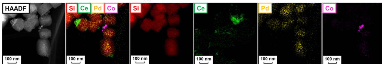
Fig. 23 STEM-EDS images of (A) 1 wt% Pd-1 wt% Co/Ce-MFI MC and (B) 1 wt% Pd-1 wt% Co/Ce-MFI HT . Reproduced from ref. 88 with permission from American Chemical Society, copyright 2022.
