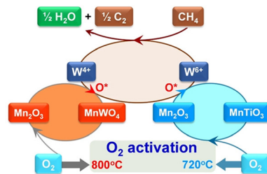
Fig. 6 Proposed catalytic cycle for OCM reaction mediated by the redox cycle \text{Mn}^{2+} \rightarrow \text{Mn}^{3+} over \text{Mn-Na}_2\text{WO}_4/\text{Ti-MWW} . Reprinted from ref. 36 with permission from The American Association for the Advancement of Science, copyright 2017.
