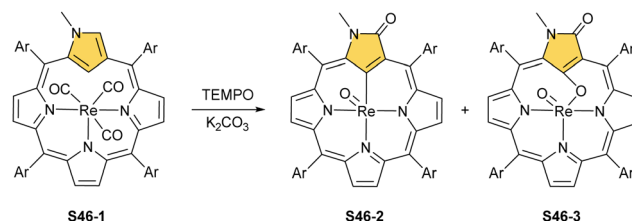
Scheme 46 Oxygenation of a rhenium(I) NCP complex S46-1 .
