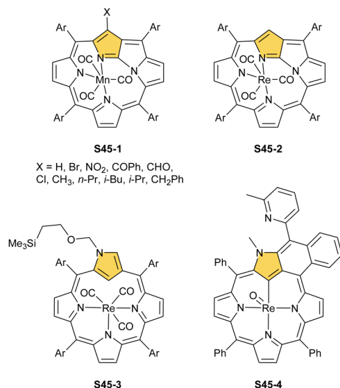
Scheme 45 Manganese(I) and rhenium(I)/(V) complexes of N-confused porphyrin derivatives.
