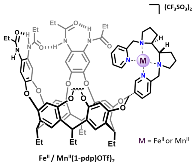
Fig. 1 Representation of cavitand-tailored bioinspired complexes \text{Fe}^{\text{II}}(\mathbf{1}\text{-pdp})(\text{OTf})_2 and \text{Mn}^{\text{II}}(\mathbf{1}\text{-pdp})(\text{OTf})_2 .
