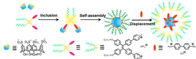
Fig. 16 Schematic diagram of substitution activated phototheranostics, and the proposed mechanism of cytoplasm-to-mitochondrial translocation of TPE-PHO \leftarrow SC4A + BZD.
