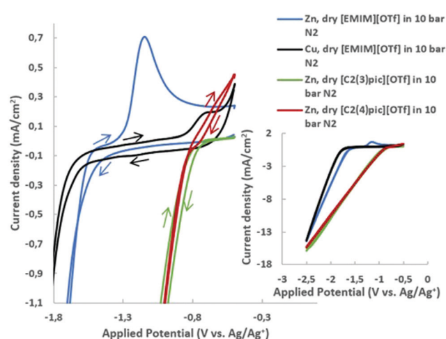
Fig. 2 Cyclic voltammograms at 45 °C carried out at 50 mV s -1 in the potential range of -0.5 V up to -2.5 V vs. Ag/Ag + (QRE) in dry [EMIM][OTf] at zinc and copper cathodes and in dry [C 2 (3)pic][OTf] and [C 2 (4)pic][OTf] at zinc cathodes in N 2 atmosphere.
