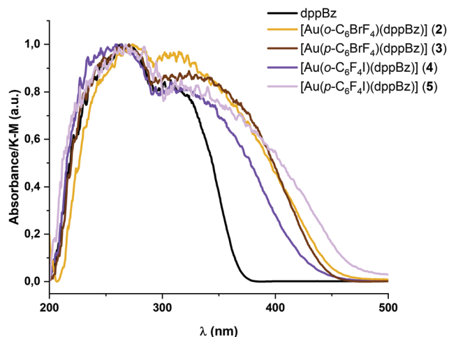
Fig. 3 Experimental UV-vis absorption spectra of complexes [Au(o-C 6 BrF 4 )(dppBz)] ( 2 ) (orange), [Au(p-C 6 BrF 4 )(dppBz)] ( 3 ) (brown), [Au(o-C 6 F 4 l)(dppBz)] ( 4 ) (purple), and [Au(p-C 6 F 4 l)(dppBz)] ( 5 ) (light purple), and the free ligand dppBz (black) in the solid state.
