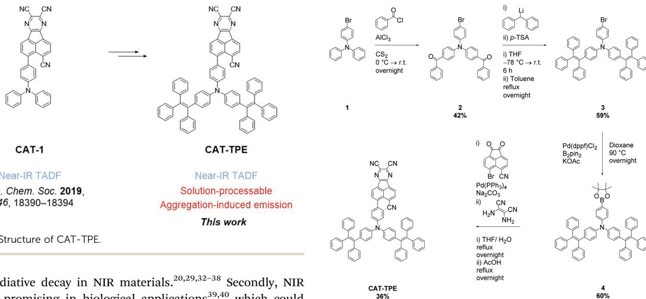
Scheme 1 Synthesis of CAT-TPE.
