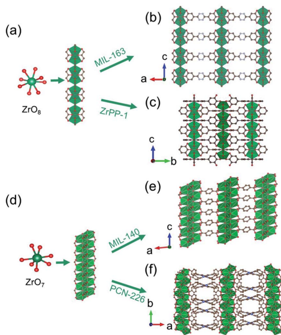
Fig. 16 (a) The infinite 1D Zr^{(iv)} -oxo chain assembled from ZrO_8 polyhedrons; (b) corresponding framework structure of MIL-163. Reproduced with permission from ref. 106. Copyright 2015, WILEY-VCH Verlag GmbH. (c) The corresponding framework structure of ZrPP-1. Reproduced with permission from ref. 34. Copyright 2018, WILEY-VCH Verlag GmbH. (d) The infinite zigzag 1D Zr^{(iv)} -oxo chain assembled from ZrO_7 polyhedrons; (e) corresponding framework structure of MIL-140. Reproduced with permission from ref. 30. Copyright 2021, WILEY-VCH Verlag GmbH. (f) The corresponding framework structure of PCN-226. Reproduced with permission from ref. 32. Copyright 2020, American Chemical Society.
