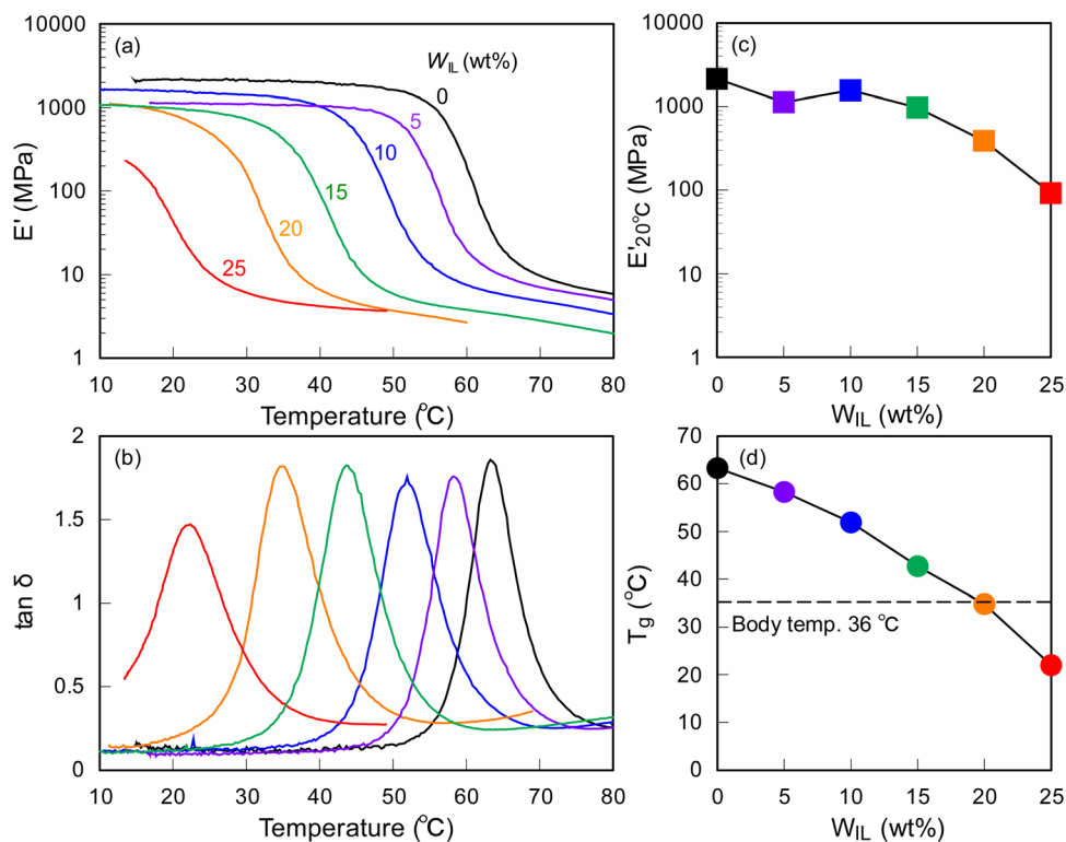
Fig. 2 Temperature dependence of (a) storage modulus ( E' ) and (b) loss tangent ( \tan \delta ) for ionic SMP gels with different W_{IL} . Dependence of (c) storage modulus at 20 ^{\circ}\text{C} ( E'_{20^{\circ}\text{C}} ) and (d) T_g of ionic SMP gels on W_{IL} .
