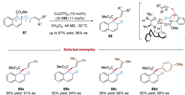
Scheme 31 Copper-catalysed enantioselective [1,3]-rearrangement.
