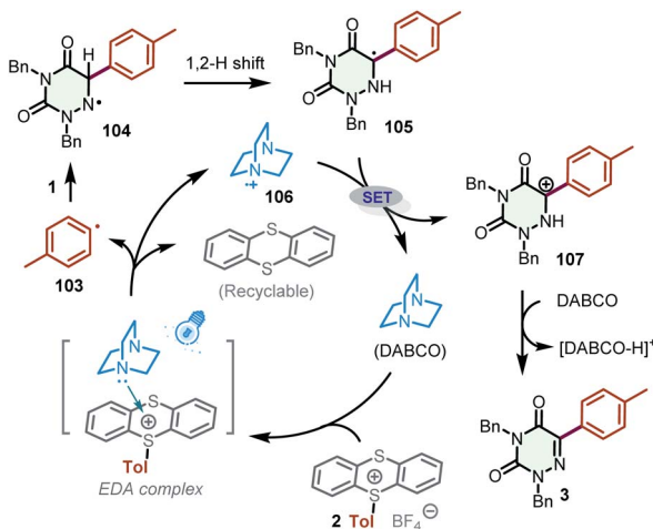
Scheme 7 Proposed mechanism.
