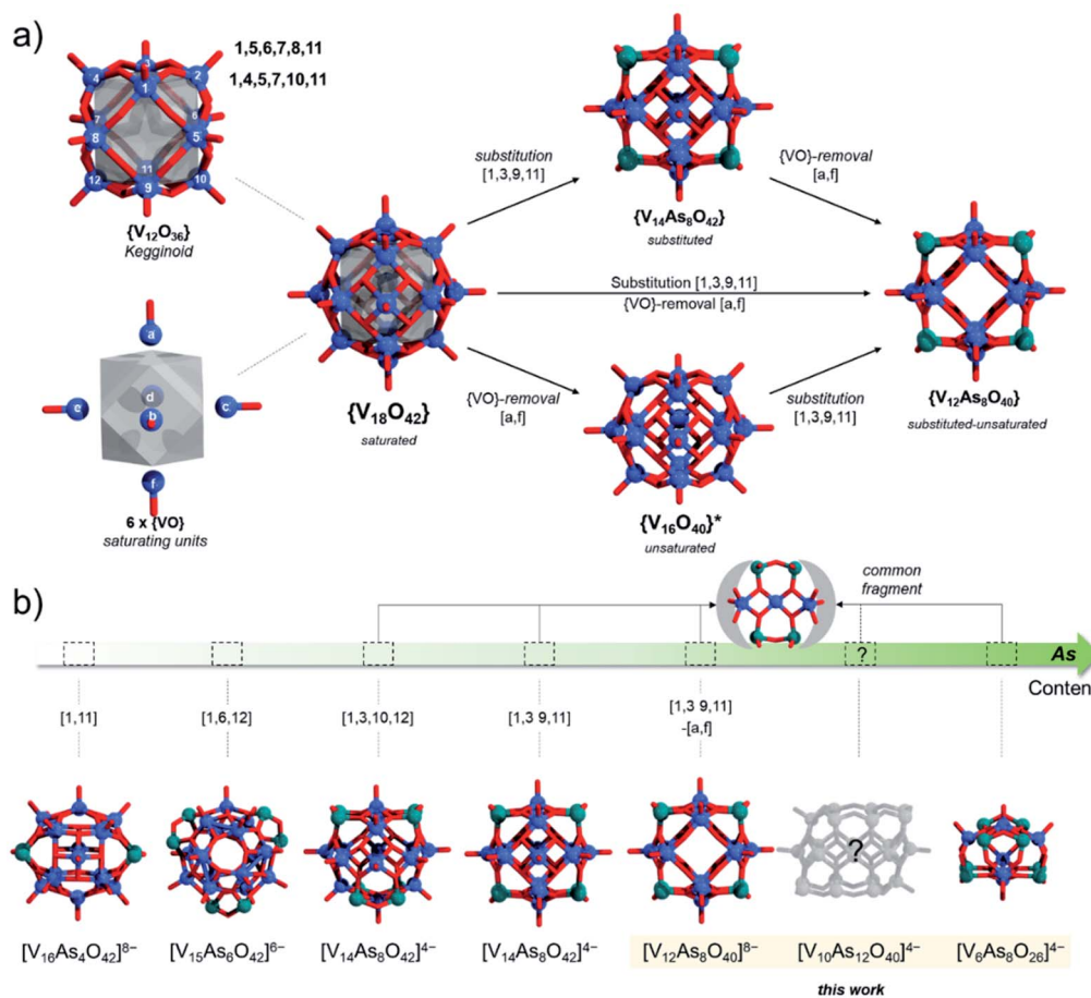
Fig. 2 Combination of ball-and-stick and schematic illustrations presenting (a) from left to right: the enumeration of the eighteen V centres in the kegginoidal \alpha - \{\text{V}_{18}\text{O}_{42}\} , the kegginoidal \alpha - \{\text{V}_{18}\text{O}_{42}\} archetype, its substituted, unsaturated and substituted-unsaturated derivatives. For \{\text{V}_{16}\text{O}_{40}\} , the experimentally known structure derives from \beta - \{\text{V}_{18}\text{O}_{42}\} ; (b) gradual ordering of the different As-POVs according to increasing arsenic content. The substitution and {VO} removal configurations from \{\text{V}_{18}\text{O}_{42}\} are provided in parentheses. Colour code: V = blue, O = red and As = green spheres.
