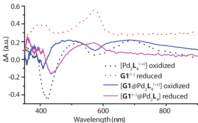
Fig. 6 Electrochemically generated difference absorption spectra for the oxidized [\text{Pd}_2\text{L}_4]^{4+} , [\text{G1@Pd}_2\text{L}_4]^{4+} and reduced \text{G1}^{(r)} , [\text{G1}^{(r)}@[\text{Pd}_2\text{L}_4]^{4+}] species (number of oxidized L units and overall charges not specified in formulas). UV-Vis spectra of samples recorded during cyclic voltammetry with a scan rate of 0.1 \text{ V s}^{-1} , Pt gauze as working electrode and \text{Ag}/\text{AgNO}_3 as reference electrode.
