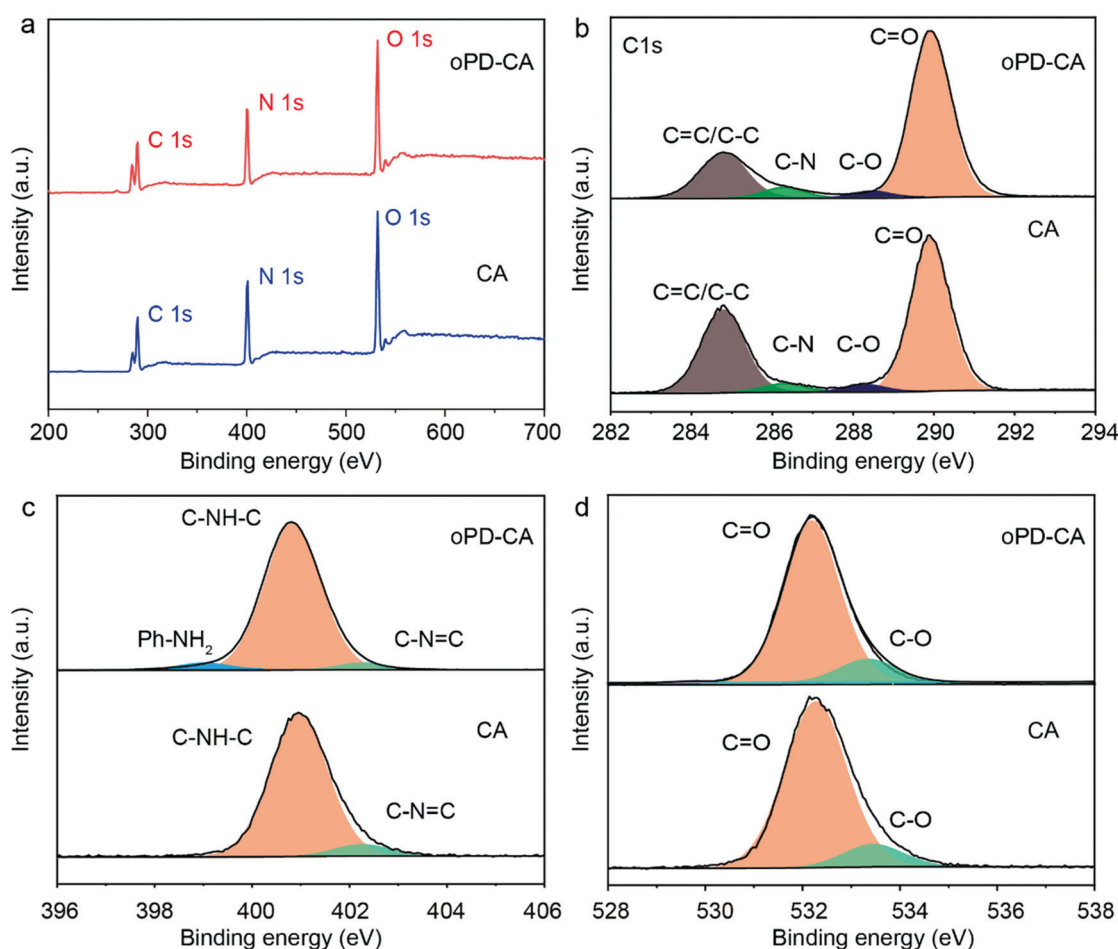
Fig. 2 XPS spectra of oPD-CA and CA for (a) survey scan, (b) \text{C}_{1\text{s}} , (c) \text{N}_{1\text{s}} , and (d) \text{O}_{1\text{s}} .
