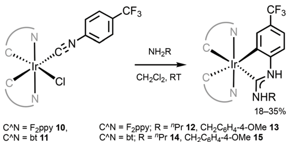
Scheme 3 Synthesis of cyclometallated Ir III -ADC complexes 12–15 . 57
