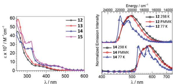
Fig. 6 (Left): UV-vis spectra of 12–15 in CH 2 Cl 2 ; (right): normalised emission spectra of 12 and 14 in CH 2 Cl 2 solution at 298 K, in CH 2 Cl 2 /toluene glass at 77 K (λ ext 310 nm), and in the PMMA film (2 wt%) at 298 K (λ ext 365 nm). Adapted with permission from ref. 57. Copyright (2018) American Chemical Society.
