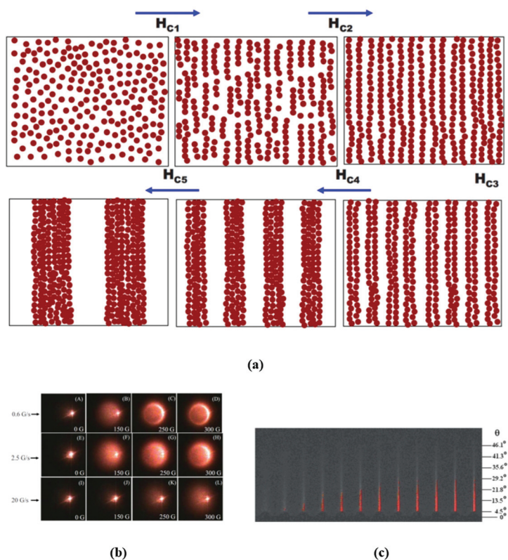
Fig. 14 Primary and secondary particle aggregation. (a) Schematic of the arrangement of magnetic nanoparticles in the dispersion before and after aggregation at different critical fields HC1, HC2, HC3, HC4, and HC5 (reproduced from ref. 257 with permission from Am. Phys. Soc., copyright 2009). (b) Light scattering patterns from the nanofluid at different magnetic field values (during decrease) on a screen placed perpendicular to the field direction of incident light for ramp rates 0.6 \text{ G s}^{-1} (A–D and M–P), 2.5 \text{ G s}^{-1} (E–H), and 20 \text{ G s}^{-1} (I–L) 253 (reproduced from ref. 253 with permission from Am. Phys. Soc., copyright 2010). (c) Time evolution of the forward scattered light in transverse configuration at several values of the applied magnetic field (reproduced from ref. 305 with permission from Royal Soc. Chem., copyright 2013).
