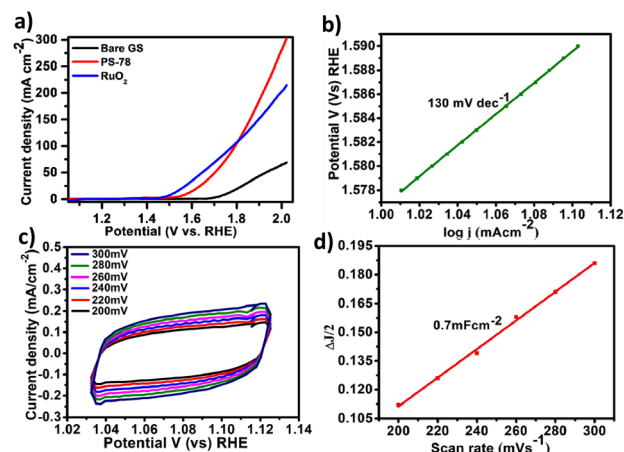
Fig. 3 (a) Polarization curves of PS-78 and the substrate (GS) at a scan rate of 5 \text{ mV s}^{-1} , (b) Tafel plot of PS-78, (c) cyclic voltammograms of PS-78 at different scan rates (200–300 \text{mV s}^{-1} ) and (d) double layer charge capacitance ( C_{dl} ) of PS-78.
