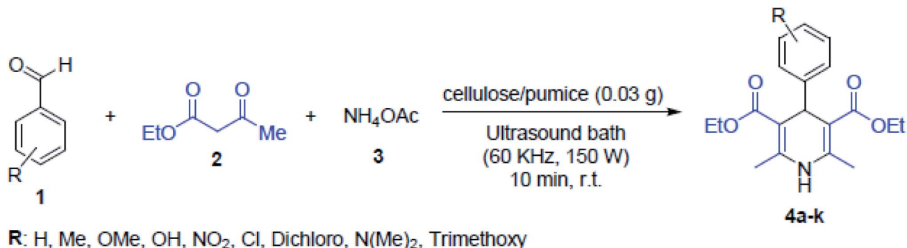
Fig. 31 Synthetic pathway for 1,4-dihydropyridine derivatives using cellulose/pumice nanocomposite catalyst via sonication at room temperature (r.t.). This figure was adapted with permission from Solid State Sciences , 2020, 101, 106141. 189
