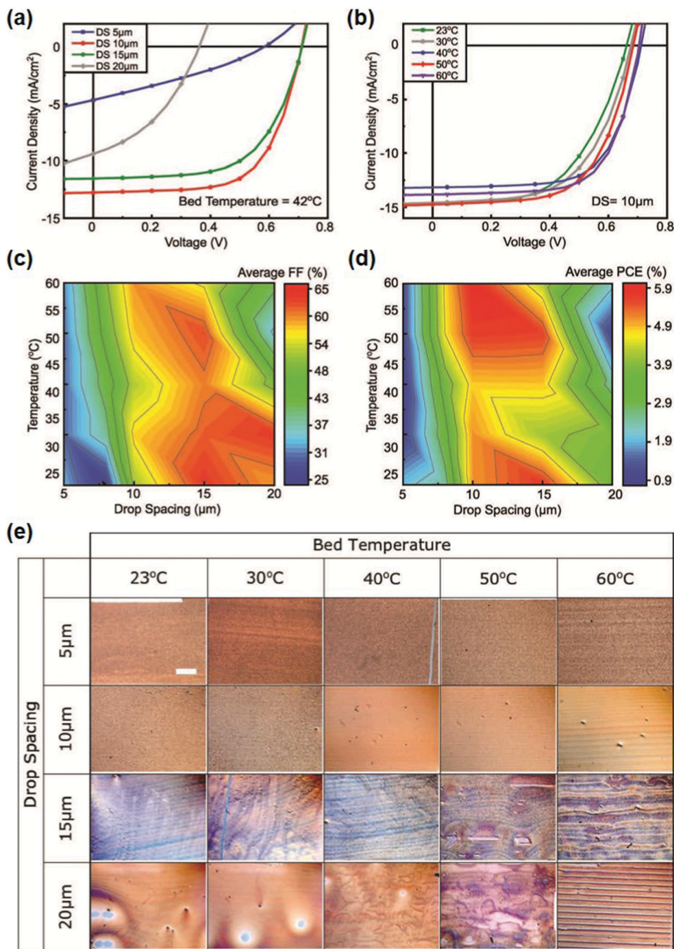
Fig. 16 (a) J-V curves of cells inkjet-printed at different drop spacing values at a constant bed temperature of 42 °C. (b) J-V curves of cells inkjet-printed with a fixed drop spacing of 10 \mu\text{m} and changing bed temperature. (c) and (d) Performance maps showing the average fill factor (FF) and PCEs of films inkjet-printed at varying drop spacing and bed temperature values. (e) Optical microscope images displaying the effects of drop spacing and bed temperature for deposition on the homogeneity and uniformity of P3HT:o-IDTBR films (scale bar = 500 \mu\text{m} ). Adapted with permission. 124 Copyright 2019, Wiley-VCH Verlag GmbH & Co. KGaA.
