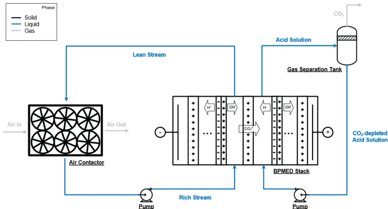
Fig. 4 An alternative aqueous alkali hydroxide solution regeneration strategy. Instead of precipitation of solid carbonates, this approach relies on a bipolar membrane electrodiolysis stack employing anion-exchange membranes to regenerate aqueous alkali hydroxide solution and to produce \text{CO}_2 . Taken from Evaluation of a direct air capture process combining wet scrubbing and bipolar membrane electrodiolysis, ref. 207, licensed under CC-BY-NC-ND 4.0.
