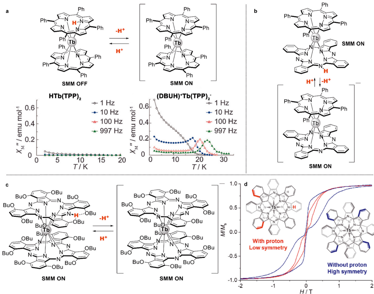
Fig. 28 (a) Proton-induced on/off switching of SMM properties ( \text{HTb}(\text{TPP})_2 and (\text{HDBU}^+)\text{[Tb}(\text{TPP})_2]^- ). (b) Protonation/deprotonation of the porphyrinato-phthalocyaninato \text{Tb}^{3+} double-decker complex \text{H}(\text{Pc})\text{Tb}(\text{TPP}) and (c) phthalocyaninato-phthalocyaninato double-decker complex \text{HTb}[(\alpha\text{-BuO})_8\text{Pc}]_2 . (d) Magnetic hysteresis curves of the protonated ( \text{HTb}[(\alpha\text{-BuO})_8\text{Pc}]_2 ) and deprotonated form ( (\text{HDBU}^+)\text{[Tb}[(\alpha\text{-BuO})_8\text{Pc}]_2]^- ) of the double-decker complex. Reproduced from (a) ref. 297 with permission from the Royal Society of Chemistry. Adapted with permission from (d) ref. 97. Copyright 2018, American Chemical Society.
