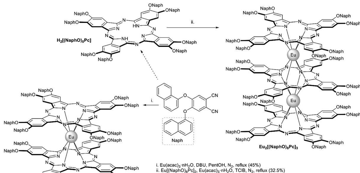
Scheme 1 Synthesis of \alpha -naphthyloxy-substituted Eu(III) bis- and trisphthalocyaninates. 38,40
