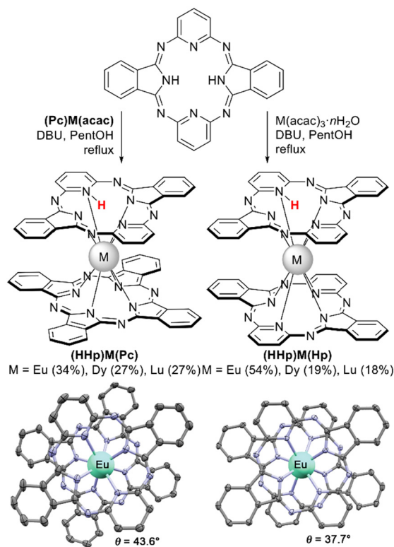
Scheme 37 Synthesis of complexes with hemiporphyrizin ligand 188,189 and X-ray structures of (\text{HHp})\text{Eu}(\text{Pc}) (CCDC GAWCAL) and (\text{HHp})\text{Eu}(\text{Hp}) (CCDC GAVXUZ). 188 Hydrogen atoms are omitted for clarity.
